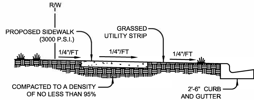
TYPICAL SECTION
